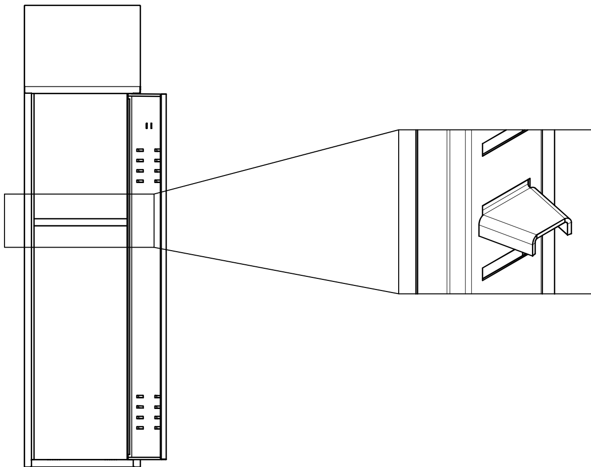
Shelf pegs
